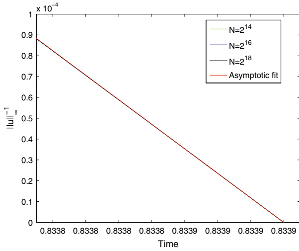
Fig. 6. The inverse of \|u\|_\infty (black) versus the asymptotic fit (red) for Initial Condition II with viscosity \nu = 0.001 . The fitted blowup time is T = 0.833919962702315 and the scaling constant is C = 1.69630372479547
