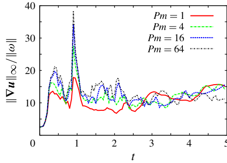
FIGURE 7. (Colour online) Plots of \|\nabla u\|_\infty / \|\omega\| versus time for Pm = 1, 4, 16, 64 .
