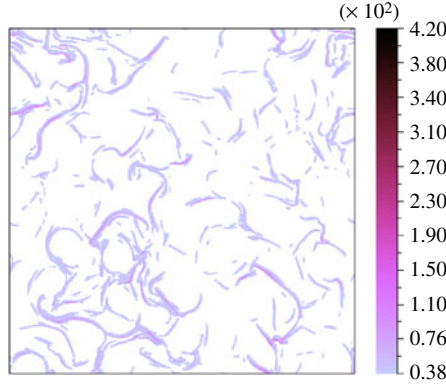
FIGURE 11. (Colour online) Velocity gradient field at t = 1 for Pm = 64 . The image is for |\nabla \mathbf{u}| \geq 2\|\omega\| \approx 3.8 \times 10^1 .
