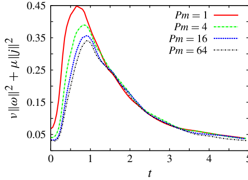
FIGURE 4. (Colour online) Total energy dissipation rates versus time for Pm = 1, 4, 16, 64 .
