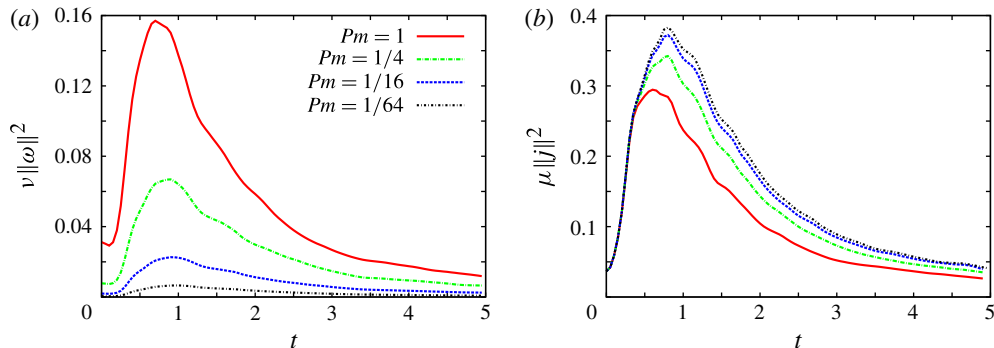
FIGURE 1. (Colour online) Kinetic (a) and magnetic (b) energy dissipation rates versus time for Pm = 1, 1/4, 1/16, 1/64 .
