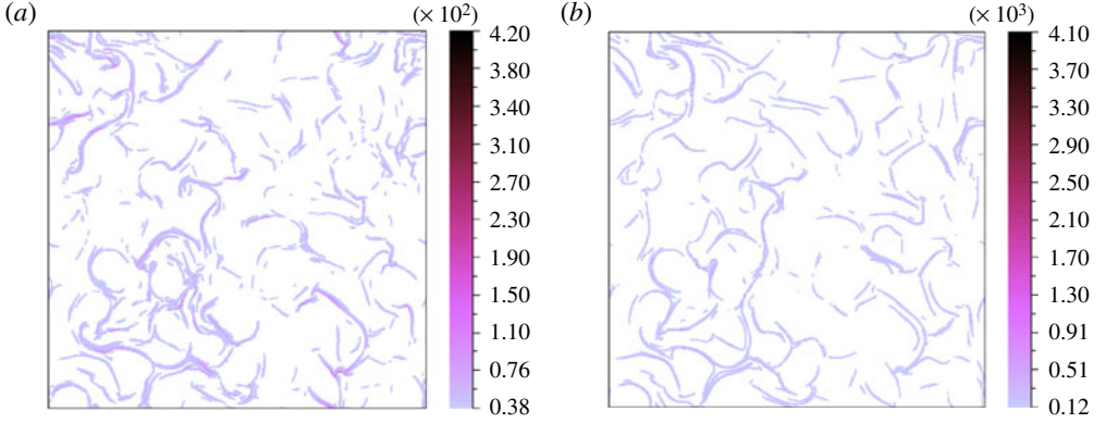
FIGURE 10. (Colour online) Vorticity (a) and current (b) fields at t = 1 for Pm = 64 . The images are for |\omega| \geq 2\|\omega\| \approx 3.8 \times 10^1 and |j| \geq 2\|j\| \approx 1.2 \times 10^2 .
