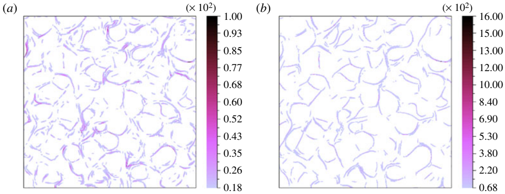
FIGURE 13. (Colour online) Vorticity (a) and current (b) fields at t = 3 for Pm = 64 . The images are for |\omega| \geq 2\|\omega\| \approx 1.8 \times 10^1 and |j| \geq 2\|j\| \approx 6.8 \times 10^1 .
