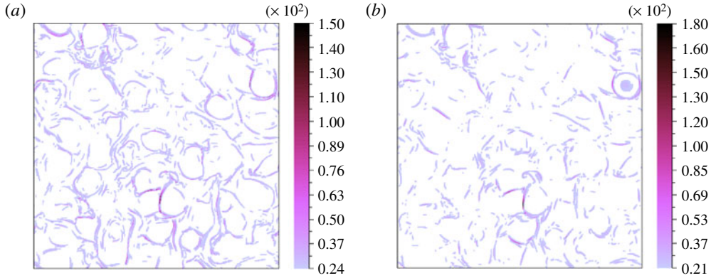
FIGURE 12. (Colour online) Vorticity (a) and current (b) fields at t = 3 for Pm = 1/64 . The images are for |\omega| \geq 2\|\omega\| \approx 2.4 \times 10^1 and |j| \geq 2\|j\| \approx 2.1 \times 10^1 .
