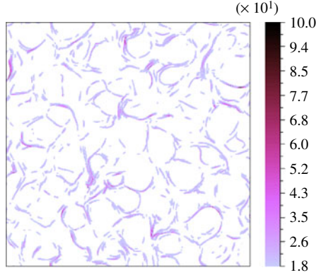
FIGURE 14. (Colour online) Velocity gradient field at t = 3 for Pm = 64 . The image is for |\nabla \mathbf{u}| \geq 2\|\omega\| \approx 1.8 \times 10^1 .
