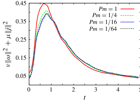
FIGURE 2. (Colour online) Total energy dissipation rates versus time for Pm = 1, 1/4, 1/16, 1/64 .
