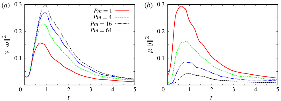
FIGURE 3. (Colour online) Kinetic (a) and magnetic (b) energy dissipation rates versus time for Pm = 1, 4, 16, 64 .
