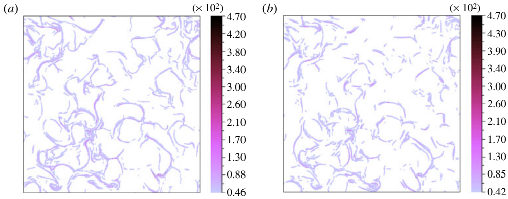
FIGURE 9. (Colour online) Vorticity (a) and current (b) fields at t = 1 for Pm = 1/64 . The images are for |\omega| \geq 2\|\omega\| \approx 4.6 \times 10^1 and |j| \geq 2\|j\| \approx 4.2 \times 10^1 .
