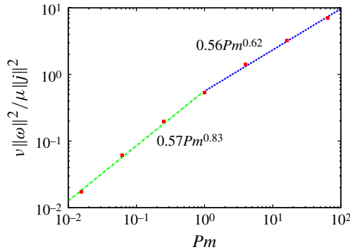
FIGURE 5. (Colour online) Ratio of peak kinetic to peak magnetic energy dissipation rates versus magnetic Prandtl number. The straight lines are best fit lines.
