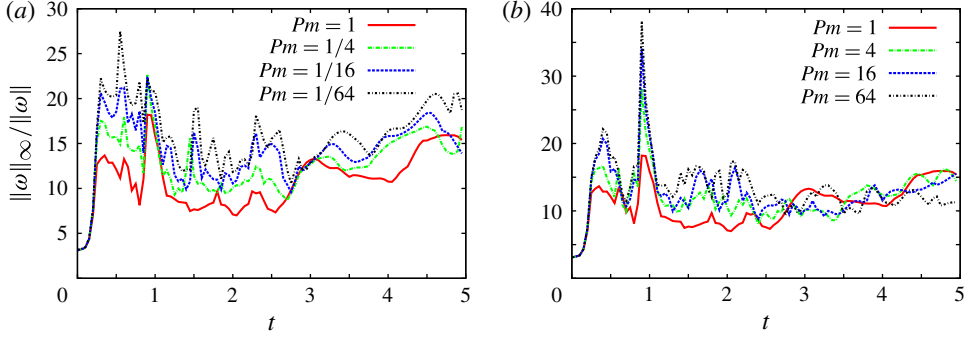
FIGURE 6. (Colour online) Plots of \|\omega\|_\infty / \|\omega\| versus time for Pm = 1, 1/4, 1/16, 1/64 (a) and for Pm = 1, 4, 16, 64 (b).
