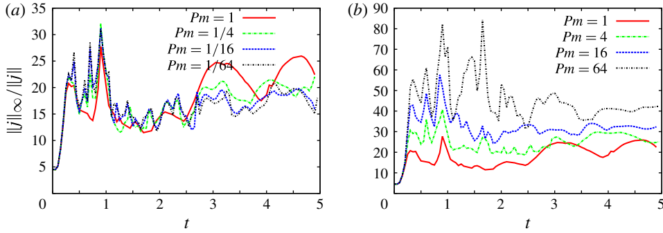
FIGURE 8. (Colour online) Plots of \|j\|_\infty / \|j\| versus time for Pm = 1, 1/4, 1/16, 1/64 (a) and for Pm = 1, 4, 16, 64 (b).
