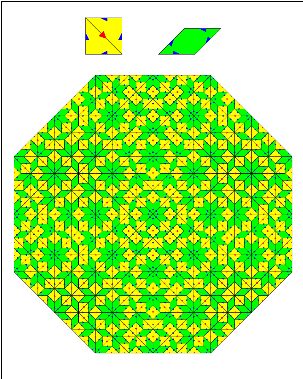
Box 4 A central patch of the octagonal Ammann-Beenker tiling The original prototiles are a square and a 45^\circ rhombus, decorated with blue arrows on the edges. For later use, the square is cut into two congruent isosceles triangles, carrying a red arrow on their common base. The orientation of arrows within each triangle is circular. Unlike the situation in the Penrose tiling, even with these arrows periodic tilings are still possible, for instance by repeating the square periodically. The octagonal patch shown belongs to the eightfold symmetric relative of the Penrose tiling, which is non-periodic and usually called the octagonal or the Ammann-Beenker tiling.
