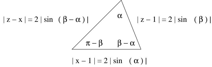
Fig. 2. We always obtain a triangle for this case.
