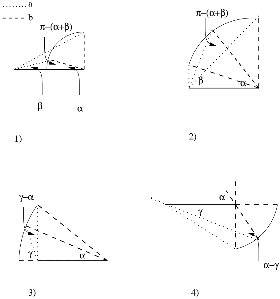
Fig. 1. 1) Case when 0 \leq b \leq 1 in the first integral. 2) Case when 1 \leq b in the first integral. 3) Case when \gamma \geq \alpha in the second integral. 4) Case when \gamma \leq \alpha in the second integral.
