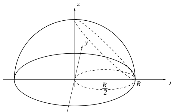
Figure 5.5: Intersection of a solid hemisphere with a cylinder
