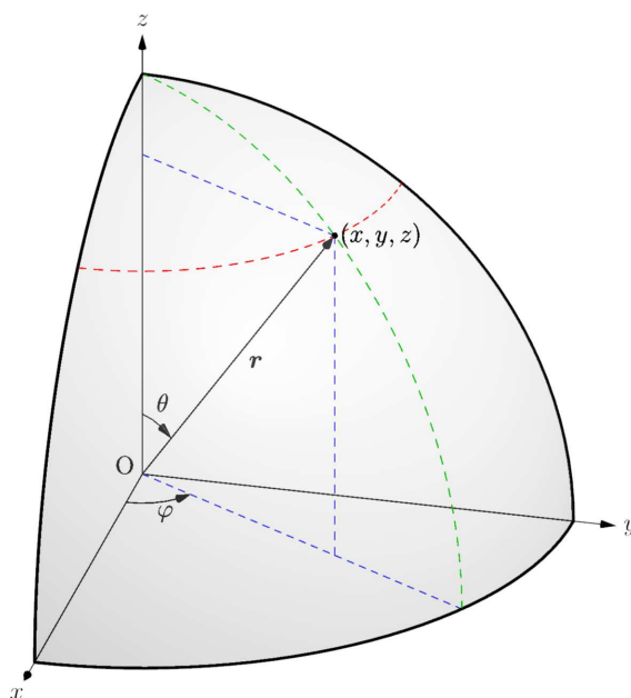
Figure 4.8: Spherical coordinates
