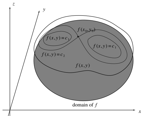
Figure 5.1: Level curves
