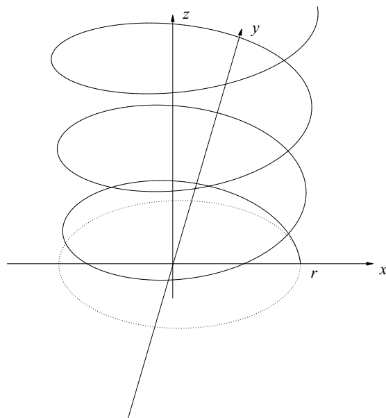
Figure 6.1: Helix
