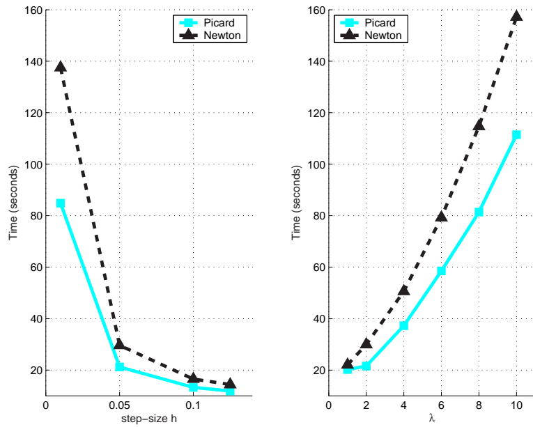
FIGURE 4.2.1. Comparison of execution time for h and \lambda for the Kepler problem
