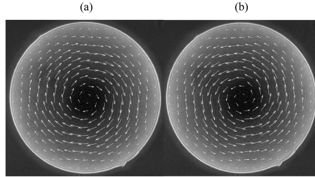
FIGURE 4. Phase-contrast image and instantaneous velocity field of giant vortices with variable direction, snapshots are taken at (a) t=10.00 and (b) t=22.00 ( https://static-content.springer.com/esm/art%3A10.1038%2Fs41586-020-03168-6/MediaObjects/41586_2020_3168_MOESM3_ESM.mp4 ).
