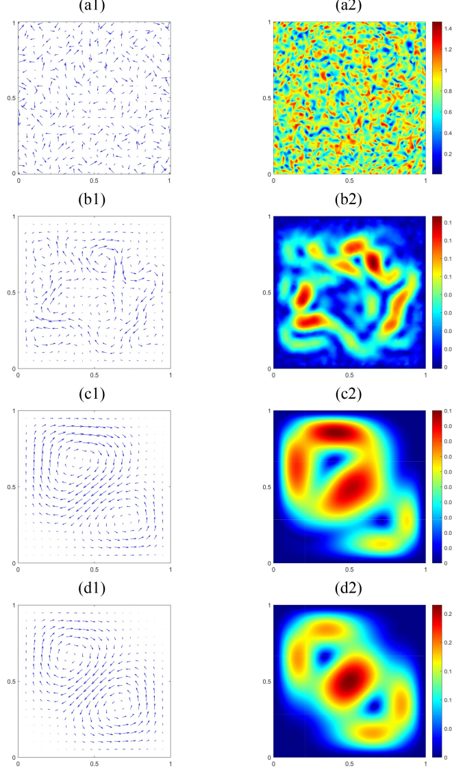
FIGURE 7. Snapshots of the velocity \mathbf{u} is taken at (a) t = 0.00 , (b) t = 0.01 , (c) t = 0.10 , (d) t = 1.00 . For each subfigure, the left is direction of velocity and the right is magnitude of velocity.
