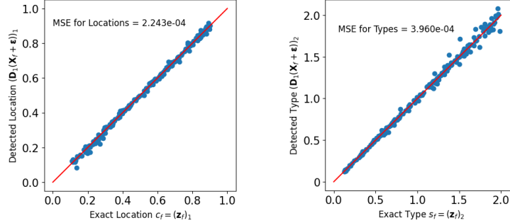
FIGURE 13. Comparisons of detected locations and exponents (or types) with the exact ones of 200 test functions in Example 4.3 using Fourier data with noise.
