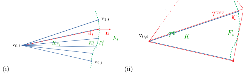
FIGURE 3. (i) Curved boundary elements for d = 2 with one curved face and vertices \mathbf{v}_{k,i} and the unit outward normal vector to F_i at x \in F_i where K_{F_i} is star-shaped and (ii) the covering mesh \mathcal{T}^{cov} , and the mesh \mathcal{T}^\# corresponding to the truth geometry with arbitrary shape boundary elements.
