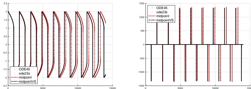
FIGURE 6. The components of the solution to the Van Der Pol's equation, with fixed step size midpoint and adaptive midpoint.
