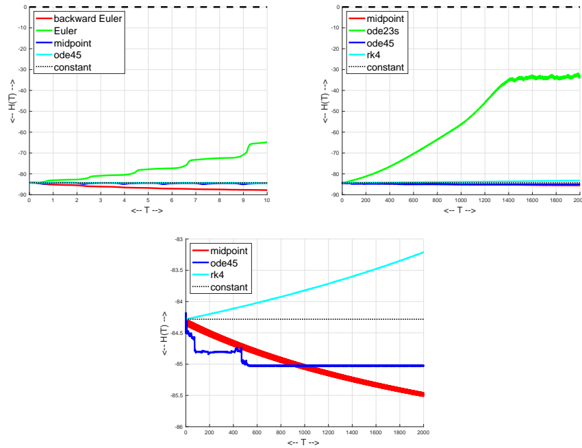
FIGURE 2. Lotka Volterra conservation.
