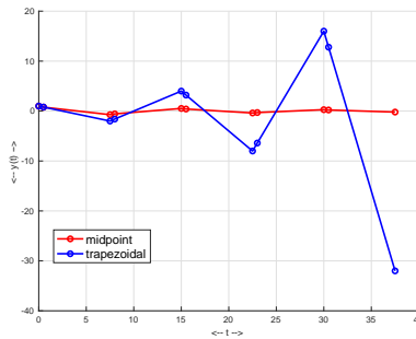
FIGURE 7. The Stetter [15] example with variable time steps: the trapezoidal method is unstable, while the midpoint method is stable.
