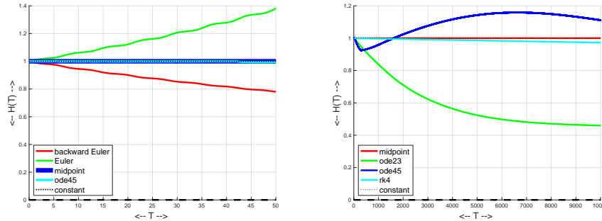
FIGURE 1. Rigid body conservation for h_1 .
