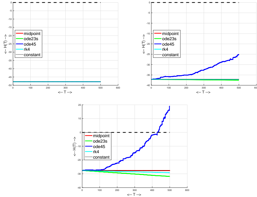
FIGURE 4. Double pendulum conservation with three energy levels.
