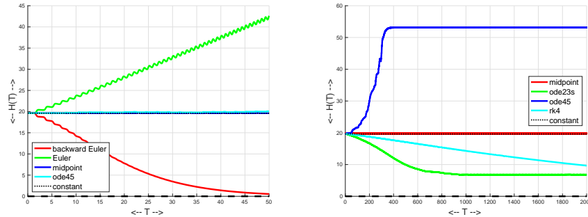
FIGURE 3. Nonlinear pendulum conservation.
