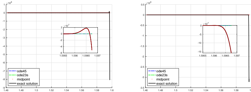
FIGURE 5. The first two components of the solution to the Lindberg’s example: ode45() , ode23s() , adaptive midpoint and the exact solution.
