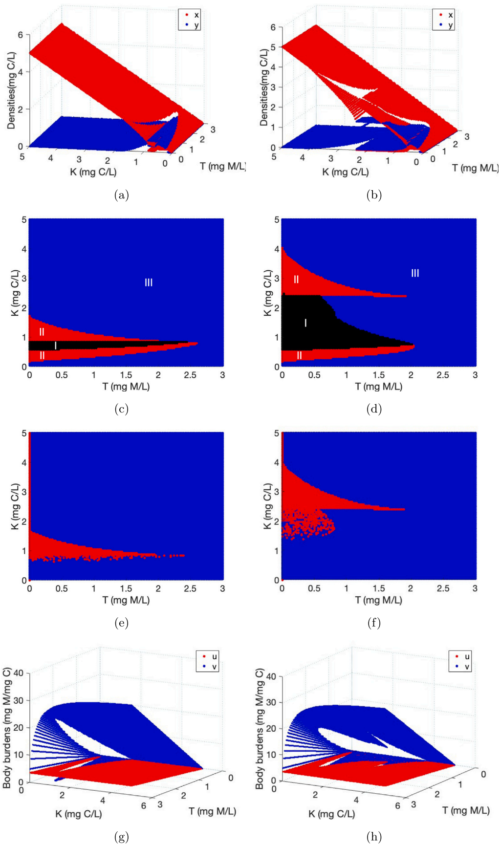
Fig. 7. (a)(b) 3D phase portraits of (2.11). (c)(d) Bifurcation diagrams for light intensity K and microplastic concentration T . (e)(f) Main limitation on grazer growth rate. (g)(h) Microplastic body burdens for producers and grazers. For the panels on the left, we choose P = 0.023 , and for the panels on the right, we choose P = 0.05 .
